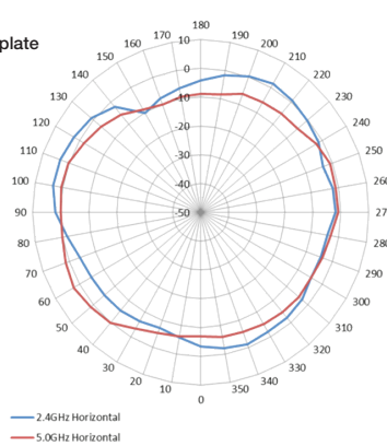
E-Plane Pattern with plastic mounting plate
