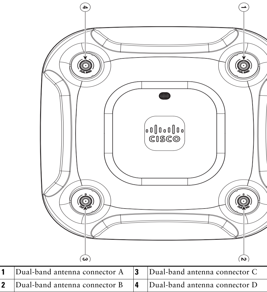
Figure 1 Access Point Ports and Connections (top)—3702E Model
